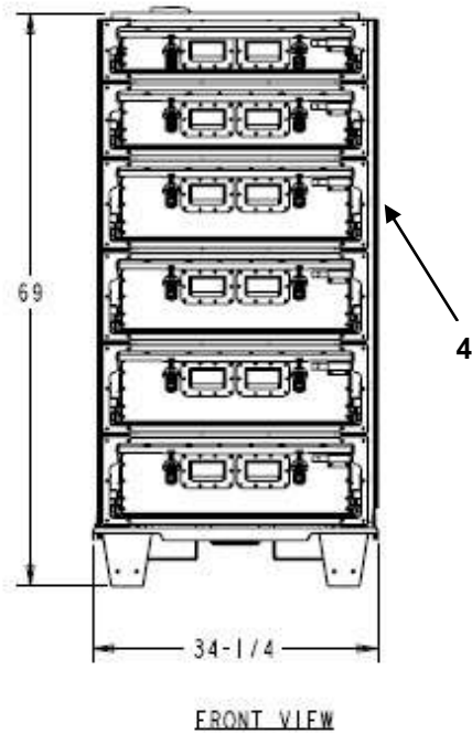
PDM CONFIGURATION #4
