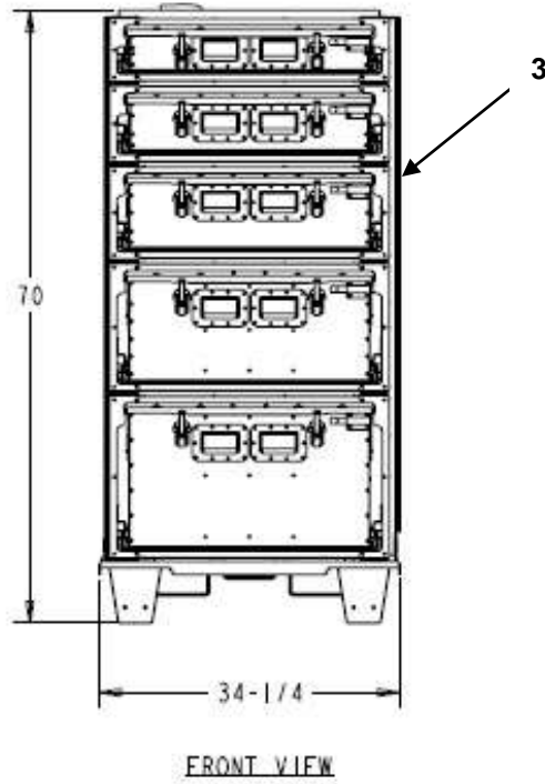
FIGURE 01 PDM CONFIGURATIONS # 01 THRU # 04
