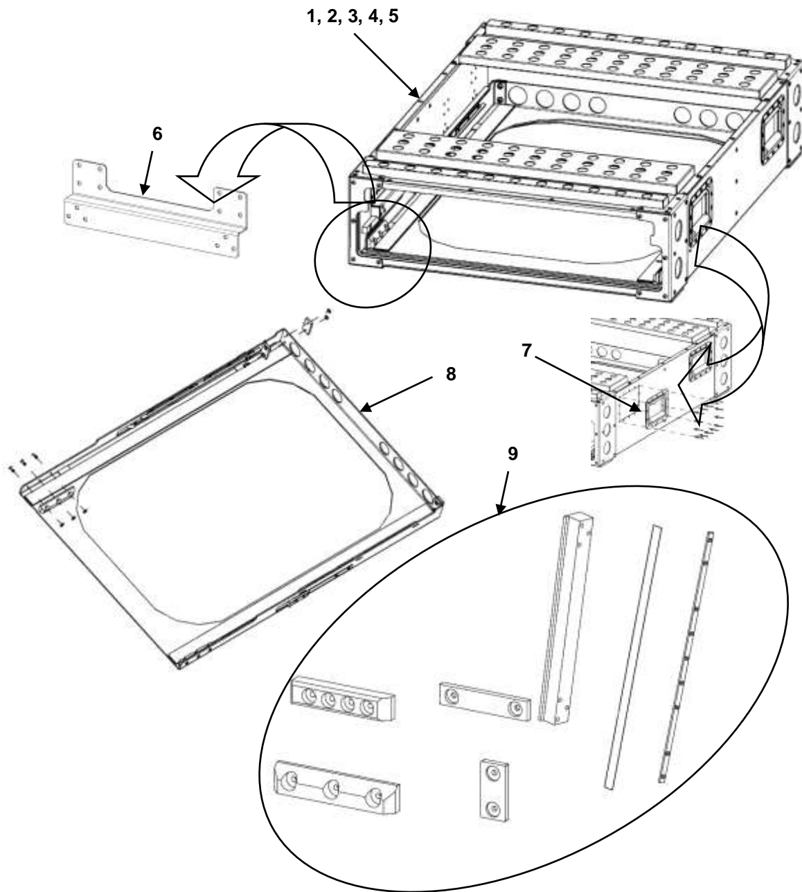
FIGURE 14 PDM 4,6,8,12,16 INCH CASES PDM TRAY AND GUIDE STRIPS
