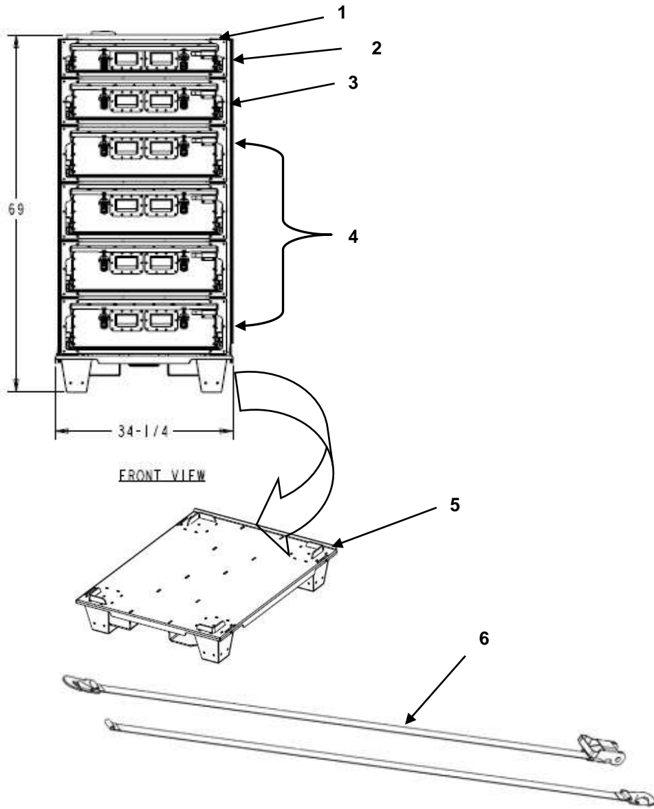
FIGURE 05 PDM CONFIGURATION # 04
