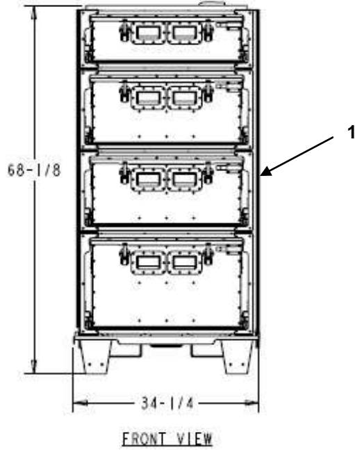
PDM CONFIGURATION #3
